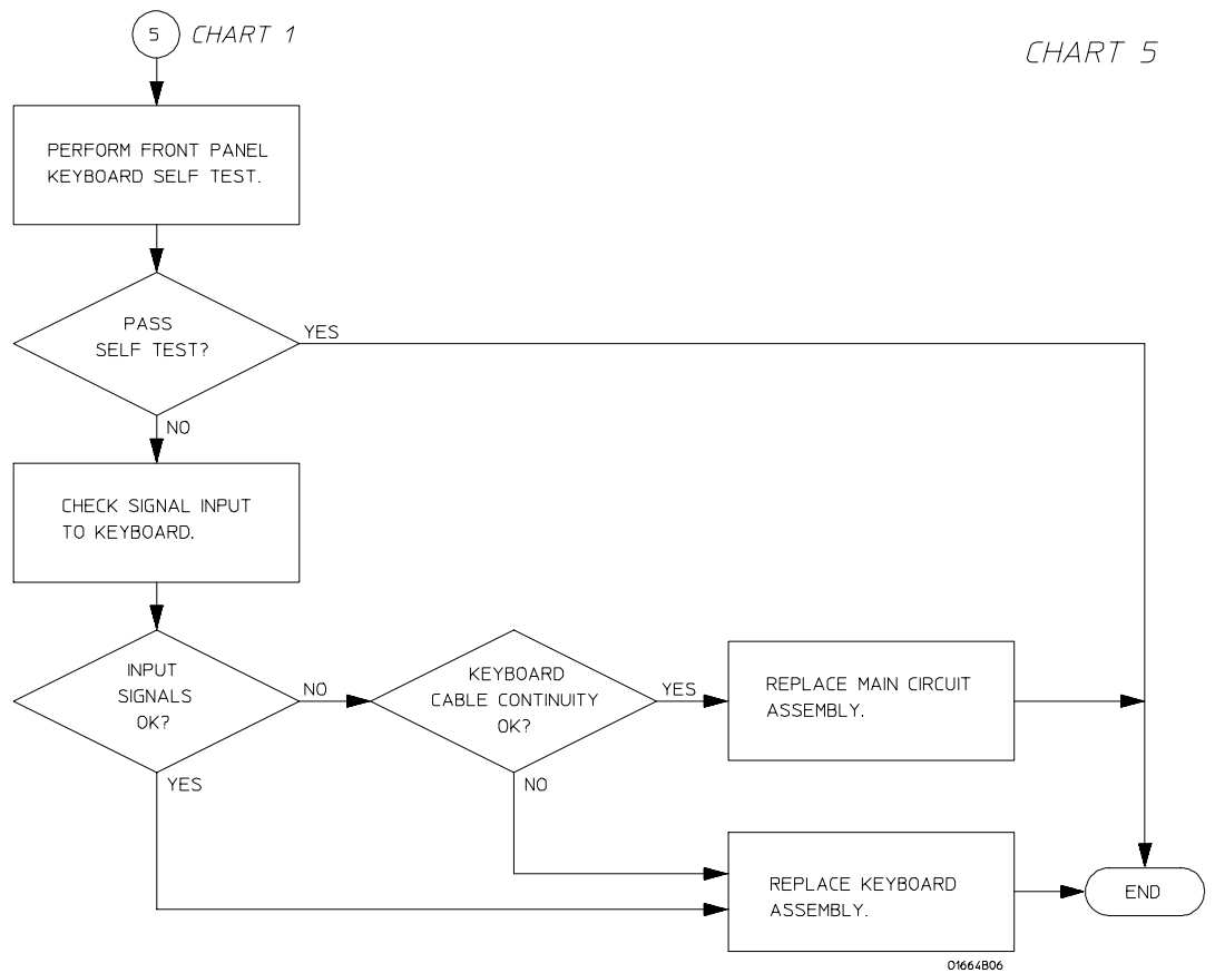
Troubleshooting Flowchart 5
