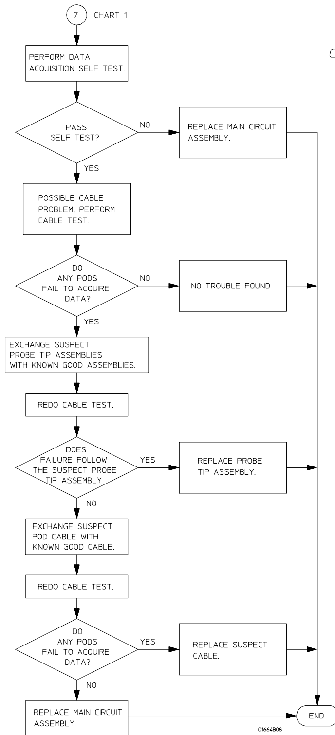
Troubleshooting Flowchart 7
