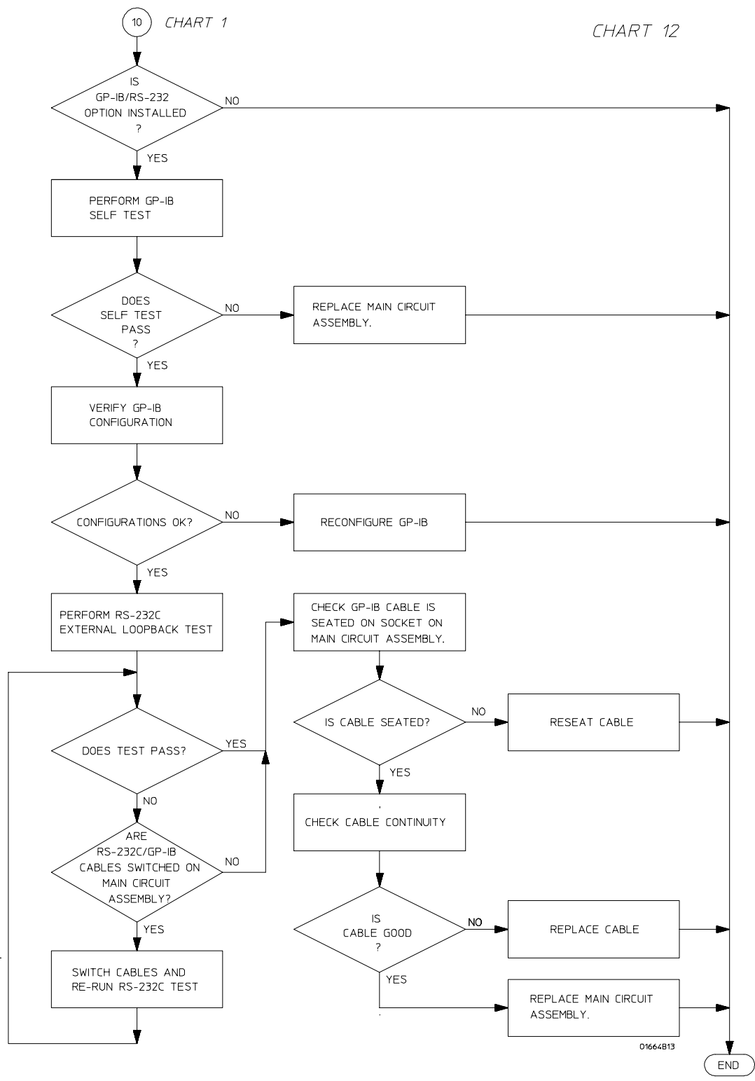
Troubleshooting Flowchart 12
