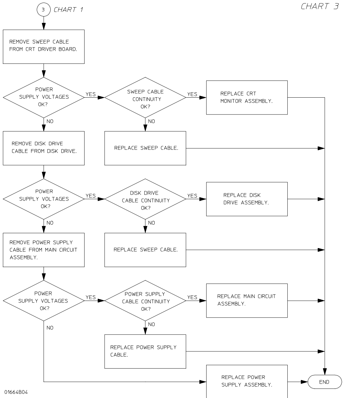
Troubleshooting Flowchart 3
