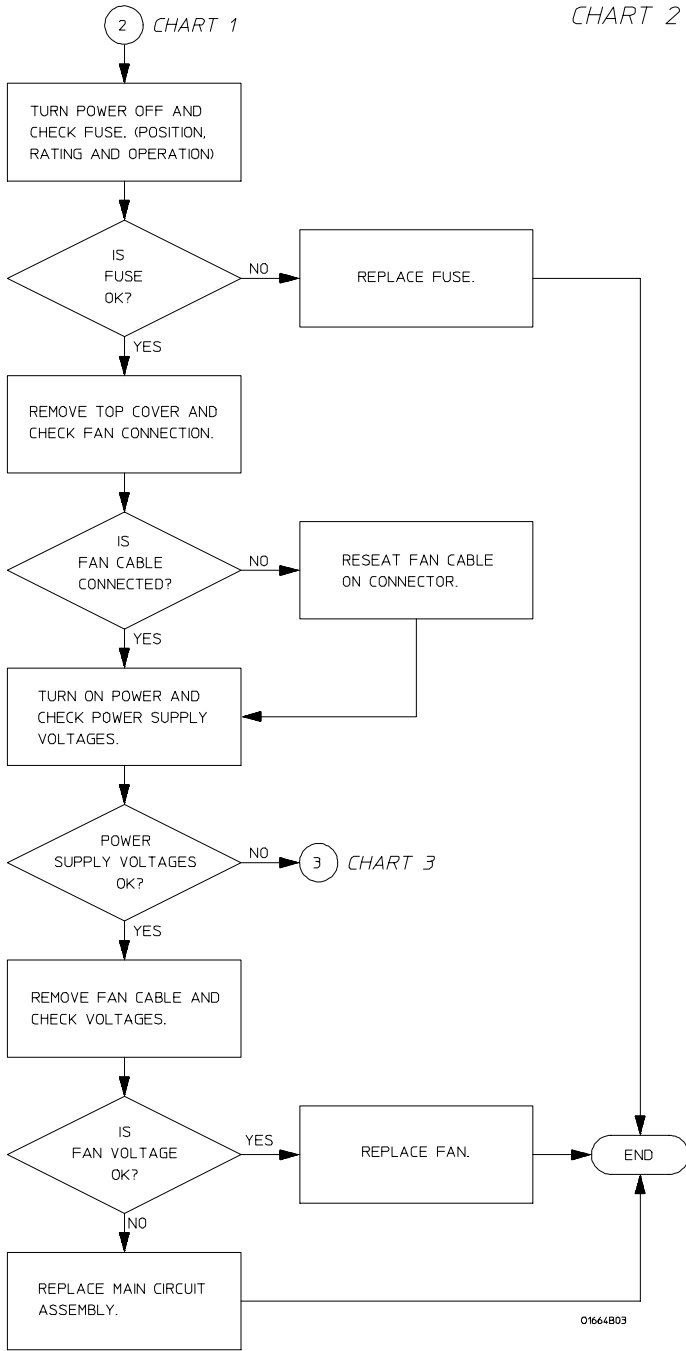
Troubleshooting Flowchart 2
