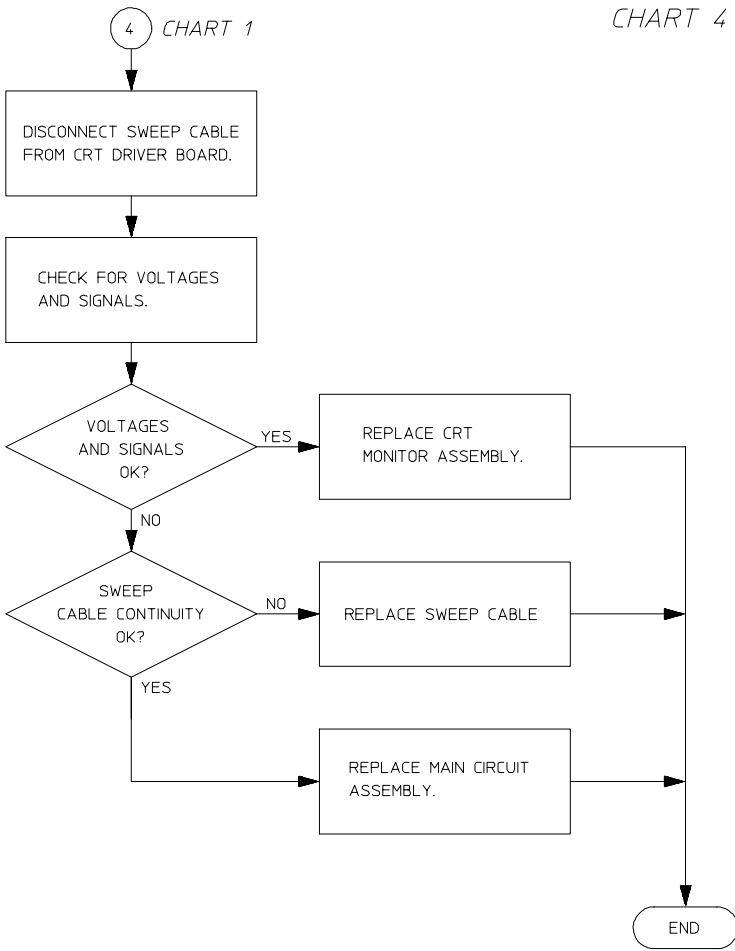
Troubleshooting Flowchart 4
