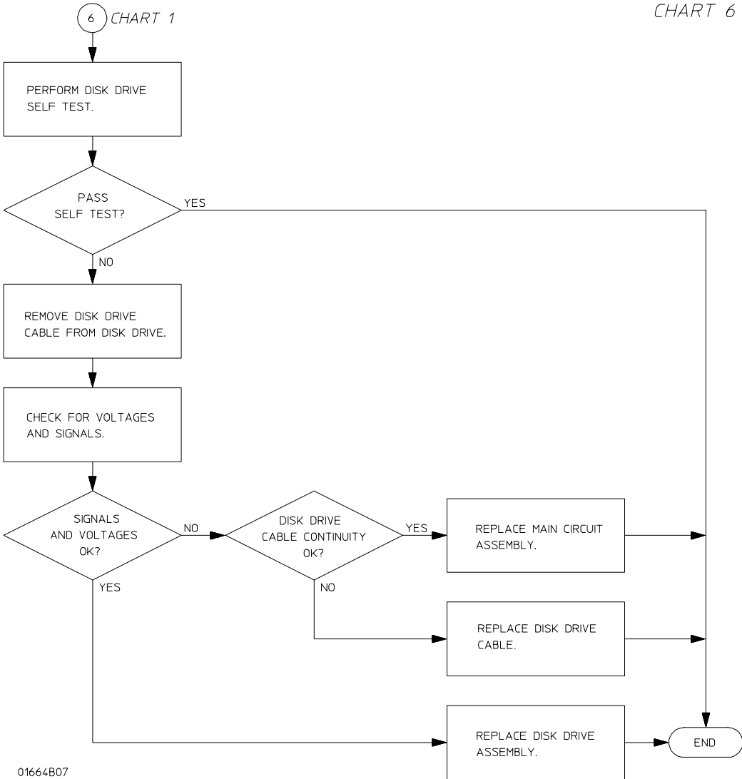
Troubleshooting Flowchart 6
