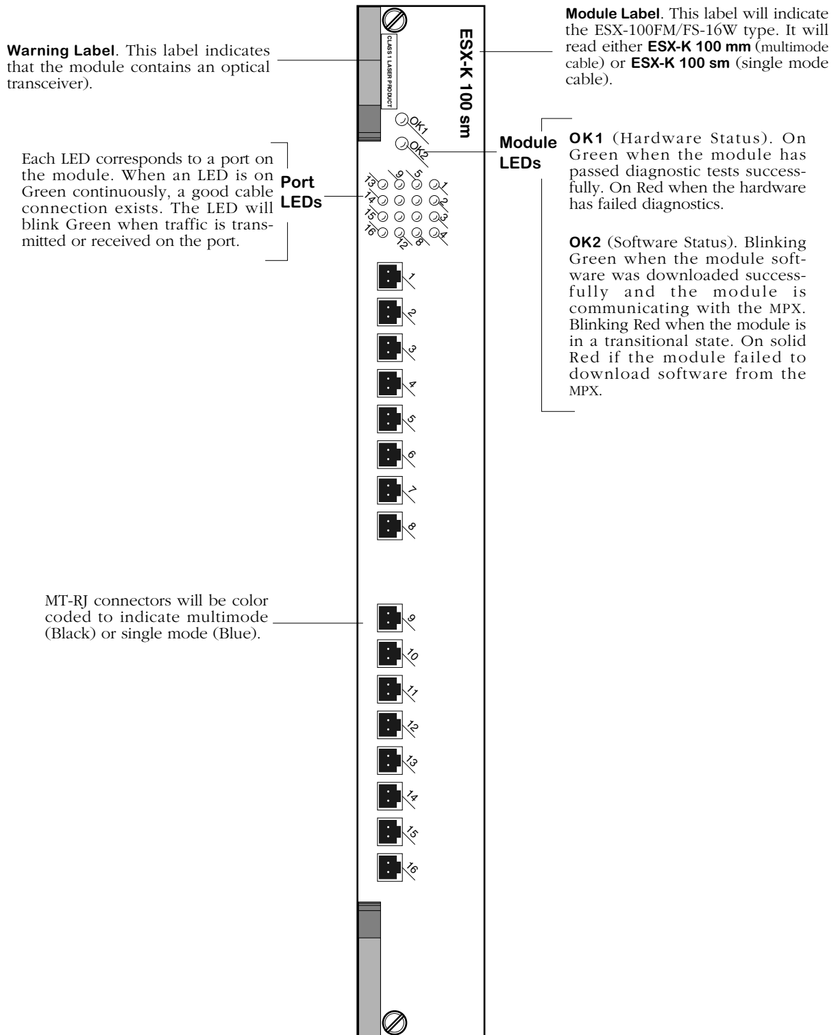
16-Port Advanced Fast Ethernet Switching Module
