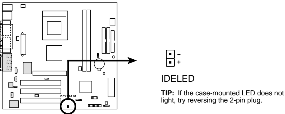
A7V133-M IDE Activity LED
