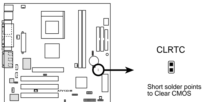
A7V133-M Clear RTC RAM
