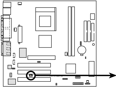
A7V133-M Wake-On-LAN Connector
