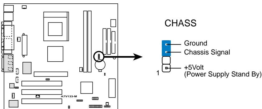
A7V133-M Chassis Open Alarm Lead
