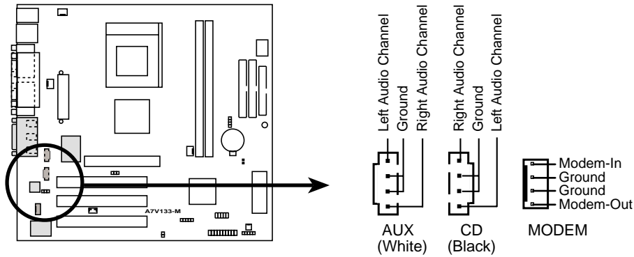
A7V133-M Internal Audio Connectors
