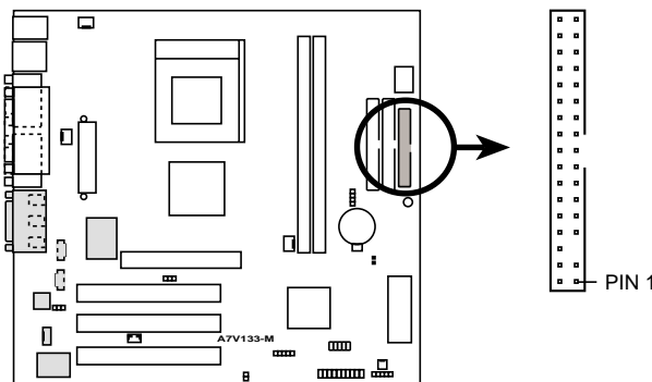
A7V133-M Floppy Disk Drive Connector
