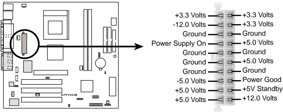
A7V133-M ATX Power Connector
