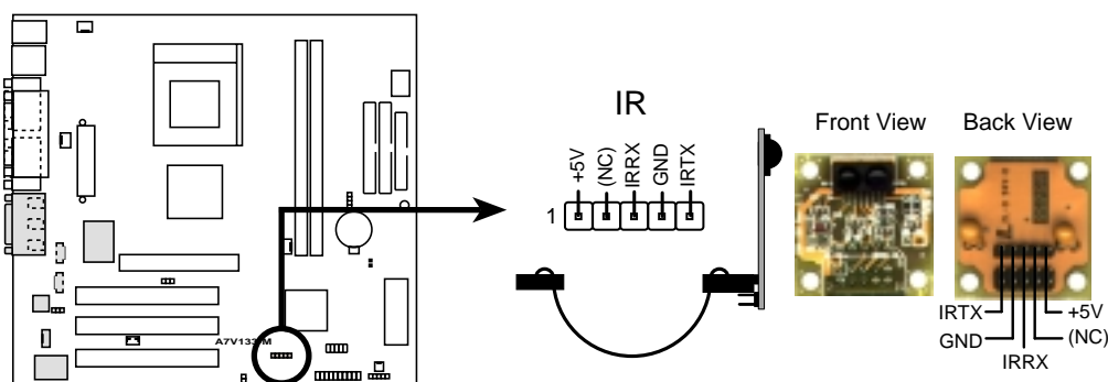
A7V133-M Infrared Module Connector
