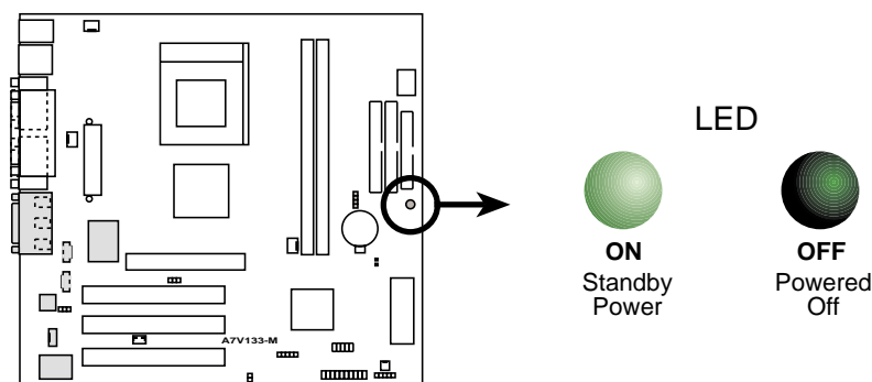
A7V133-M Onboard LED
