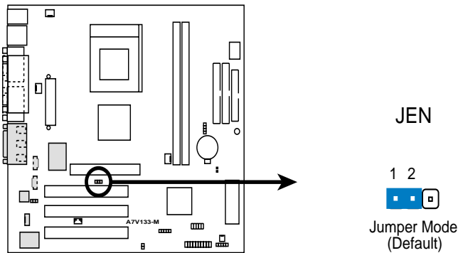
A7V133-M JumperFree™ Setting
