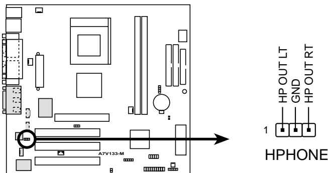
A7V133-M Headphone Connector
