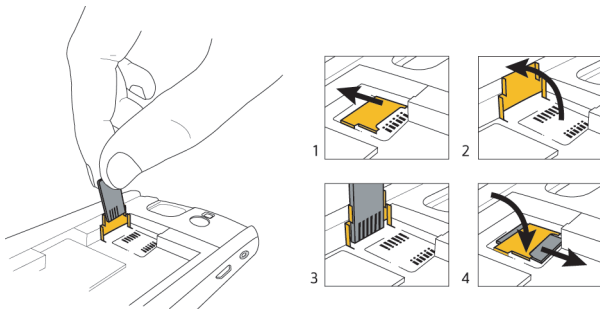
Figure 10. Insert the media card
