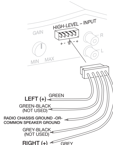
High Level (Speaker Input) Wiring
