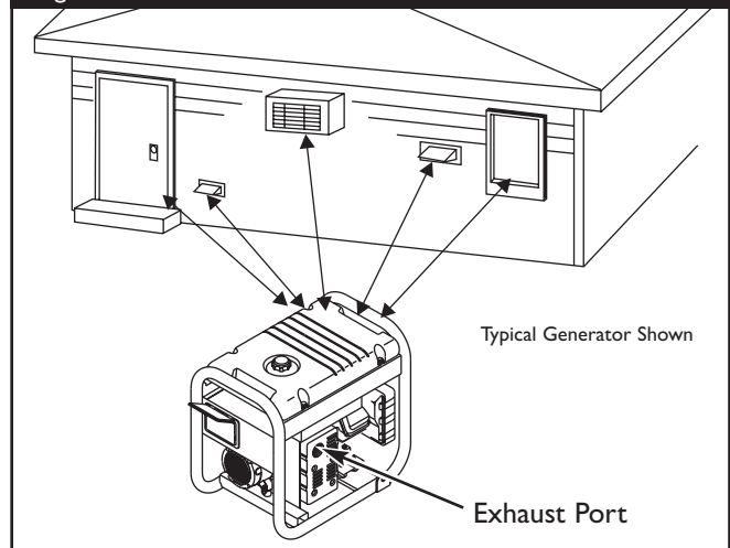
Figure 2 — Generator Clearance
