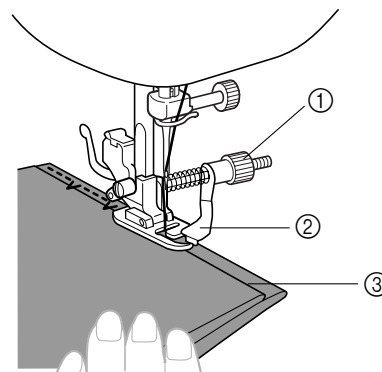
① Screw / Tornillo ② Guide / Guía ③ Folded hem / Dobladillo
