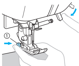
① Presser foot locking pin (black button)
