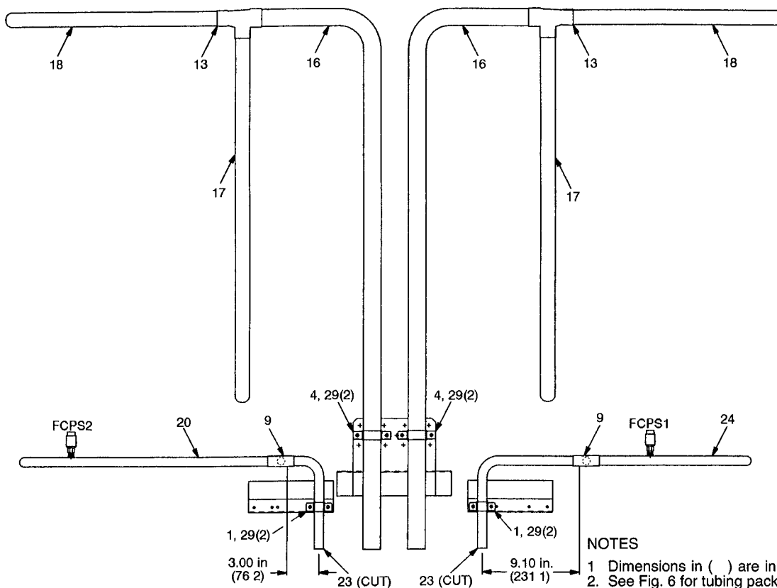
Fig. 21 — 50/50% Coil Circuiting; 074 Units
