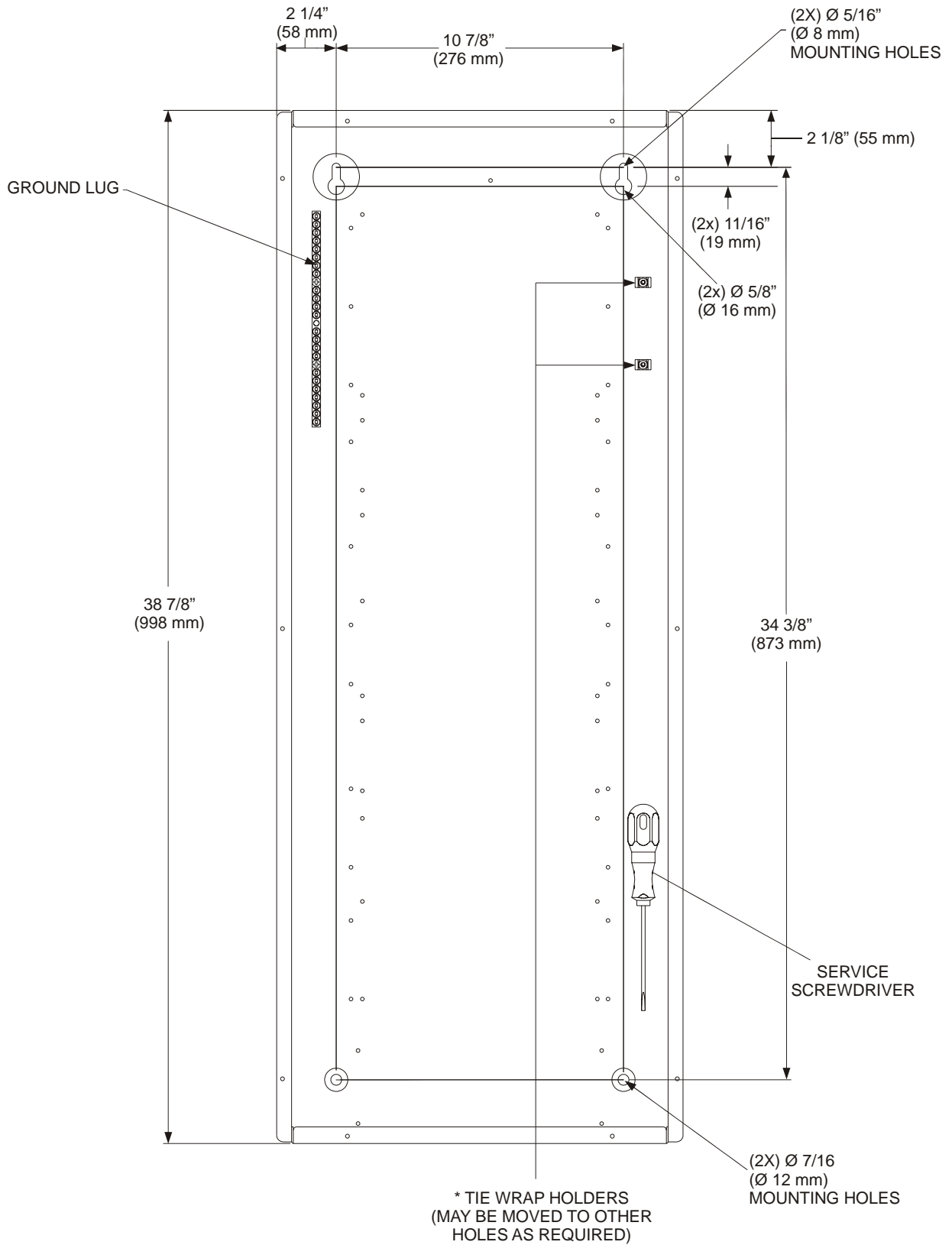
Dimensions of GLPX-HSW-FT-20, -24, -28, -32 Power Switching Cabinets (Internal View)
