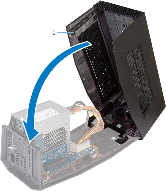
1 cover
