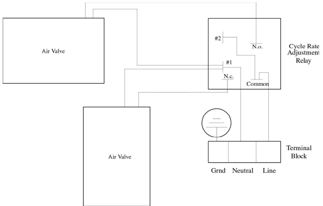
Fig.1 - Electrical Diagrams
