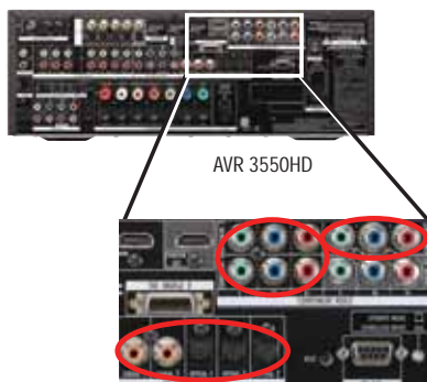
Figure 25 – Connecting a Component-Video-Equipped Recorder
