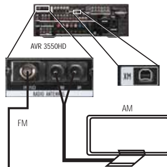
Figure 19 – Antenna Connections
