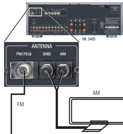
Figure 11 – Antenna Connections
