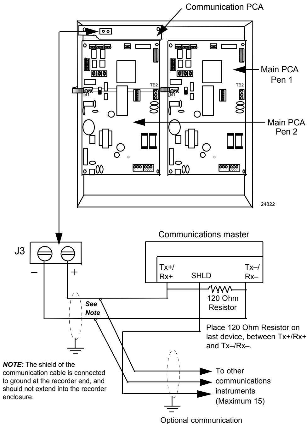
Figure 2-13 Communication Wiring
