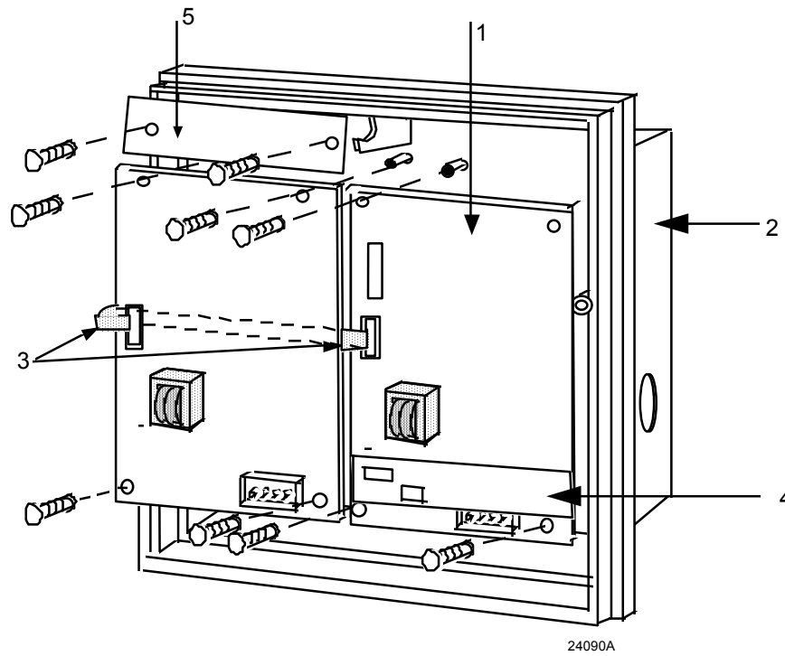
Figure 9-3 Recorder Components
